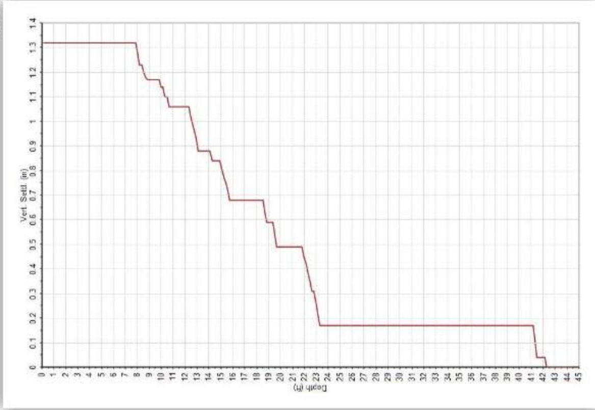
LIQUEFACTION RESULTS Trembley Lane, Watsonville
